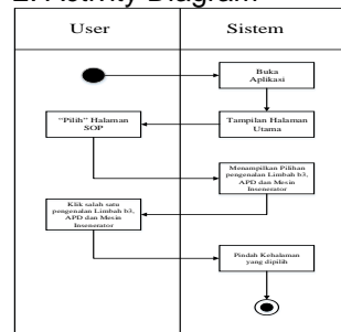
Gambar 4. Activity Diagram Sumber : Data Penelitian, 2023
