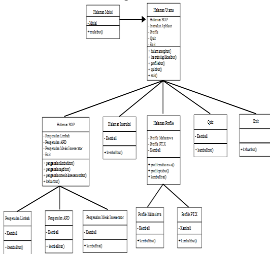
Gambar 6. Class Diagram Sumber: Data penelitian, 2023
