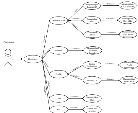
Gambar 3. Use Case Diagram Sumber : Data Penelitian, 2023
